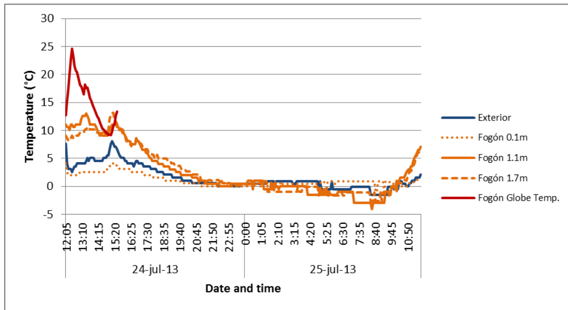
Figure 25: Simultaneous measurements of dry-bulb temperature and globe temperature at different heights. Fogón of Don Crescencio 24 th -25 th July 2013 (Winter)
