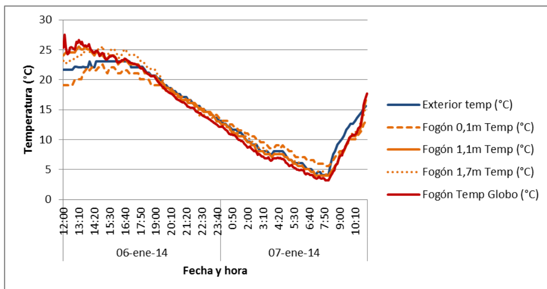
Figure 26: Simultaneous measurements of dry-bulb temperature and globe temperature at different heights. Fogón of Don Crescencio 6 th -7 th January 2014 (Austral Summer)
