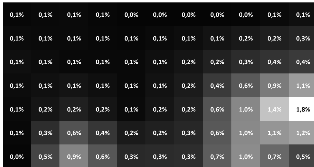
Figure 24: Distribution of daylight factor within the fogón of Don Crescencio 25 July 2014
